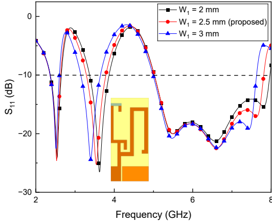
Fig. 7. Simulated results of antenna reflection coefficient with various values of W_1 .
