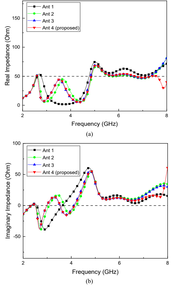
Fig. 3. Model impedance of the four proposed antenna stages. (a) real part and (b) imaginary part.
