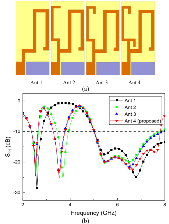
Fig. 2. (a) Evolution of antenna designs to the proposed model, (b) analysis of S_{11} responses from the evolution of the proposed antenna model.
