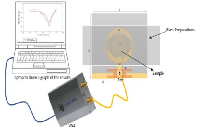
Fig. 1. RSCR Sensor and Measurement Scenario
