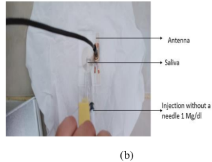
Fig. 2 (a) Sensors measurement process for detecting glucose levels with saliva samples using a vector network analyzer (VNA), (b) Injection saliva sample on flexible sensor process
