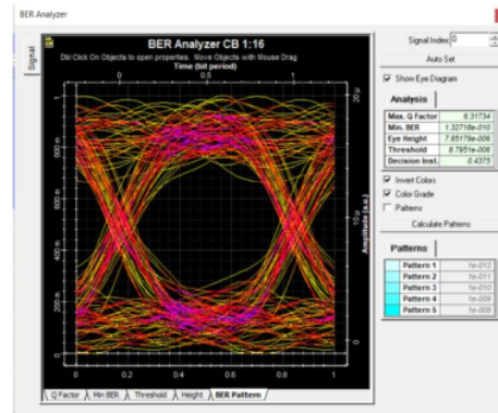
Figure 13. BER analyzer customer base method splitter scenario 1:16
