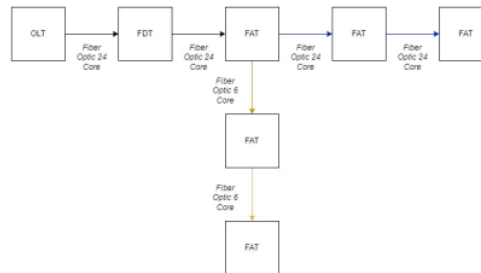
Figure 3. Block diagram of the Branching method
