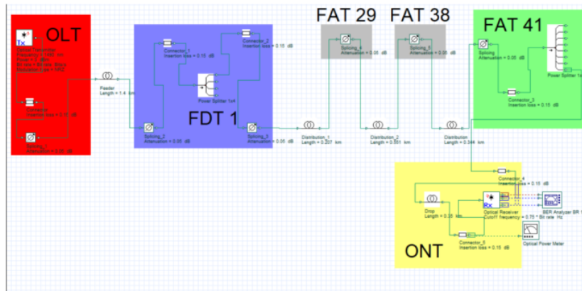
Figure 7. Branching simulation circuit
