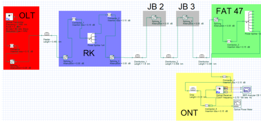
Figure 6. Customer Base simulation circuit
