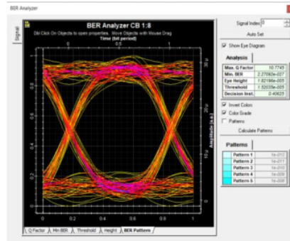
Figure 12. BER analyzer customer base method splitter scenario 1:8
