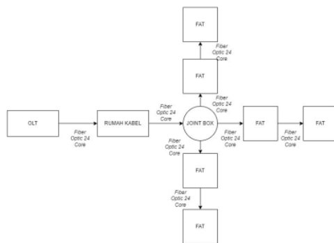
Figure 2. Block diagram of the Customer Base method
