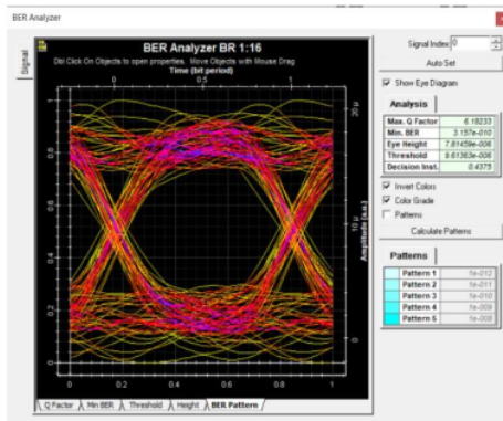
Figure 15. BER analyzer branching method splitter scenario 1:16
