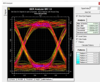
Figure 14. BER analyzer branching method splitter scenario 1:8
